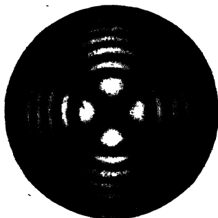
FIG. 59.—The Two Optic Axes coincident in the Centre of the Figure, two or three Minutes from the commencement. Temperature of Crystal 91^{\circ} C.
